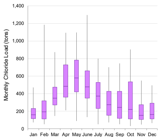
Figure 9: 2001 – 2019 Monthly Chloride Loads in Bassett Creek
