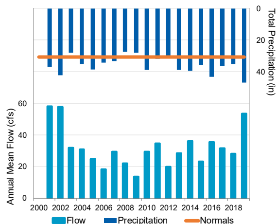
Figure 4: Annual Mean Flow and Precipitation for Bassett Creek
