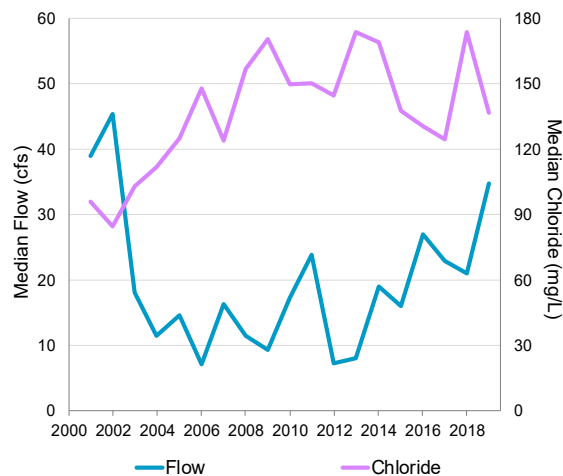
Figure 5: Annual Median Flow and Chloride Concentration in Bassett Creek
