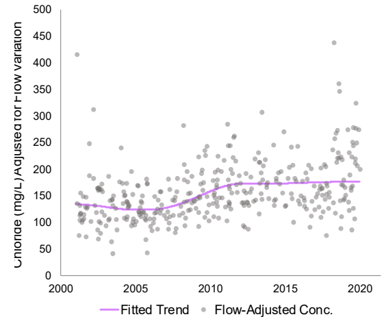
Figure 6: Flow-Adjusted Trends for Chloride Concentration in Bassett Creek
