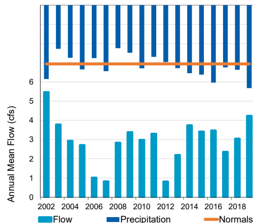
Figure 4: Annual Mean Flow and Precipitation for Fish Creek
