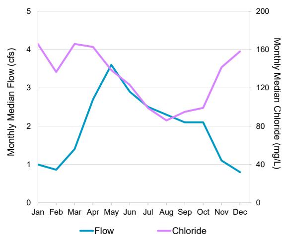
Figure 8: Monthly Median Flow and Median Ambient Chloride Concentrations in Fish Creek
