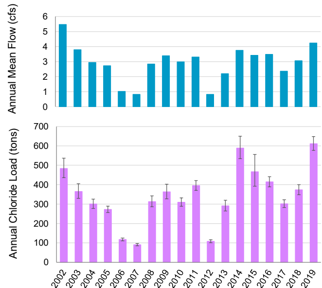
Figure 7: Annual Chloride Loads in Fish Creek (Error bars = 95% Confidence Interval)
