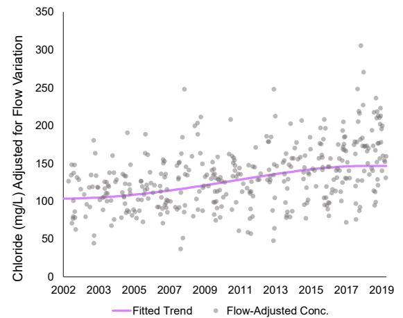
Figure 6: Flow-Adjusted Trends for Chloride Concentration in Fish Creek
